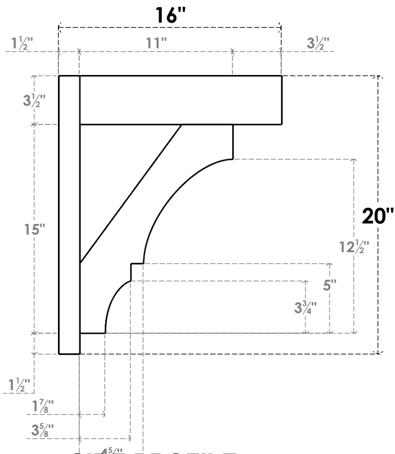
SIDE PROFILE
