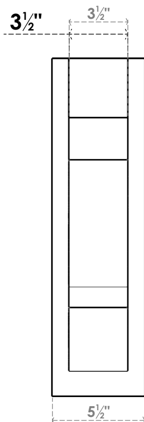
FRONT PROFILE
